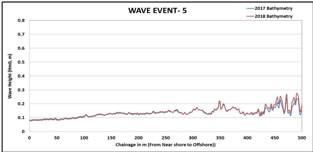
Figure 3-42 Variation of wave height from inner harbour to entrance (Hm0, m) for Wave Event - 5
