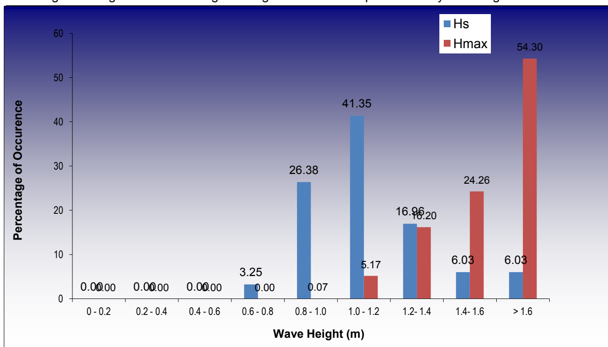
Figure 19 – Histogram of wave height (1 st to 31 st May 2019)
